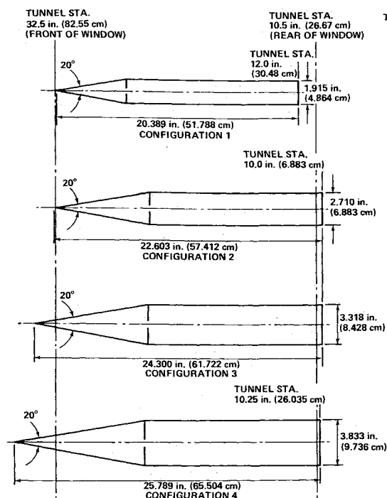
Fig. 1 Model dimensions and test locations for the five configurations.
