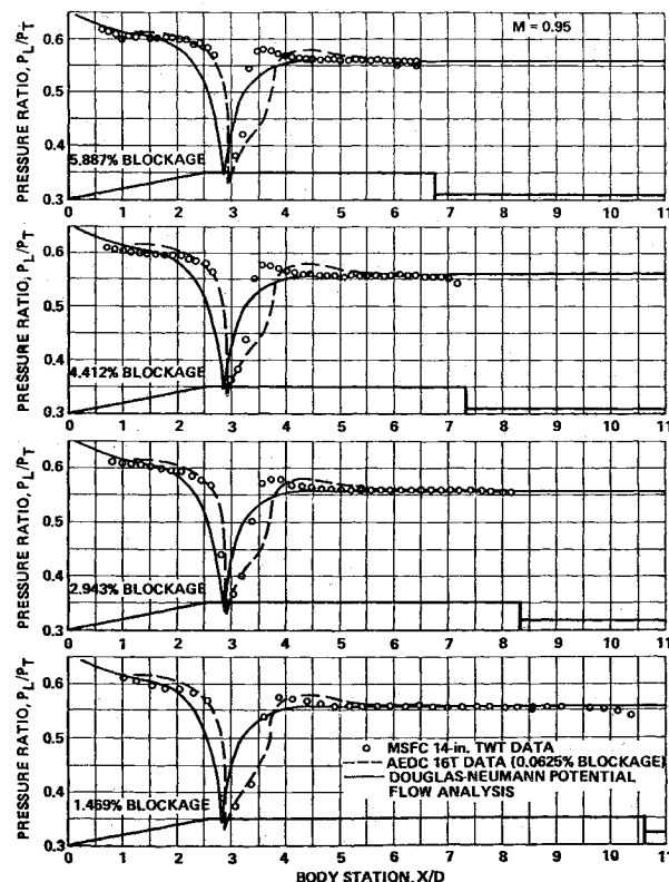
Fig. 3 Pressure distributions on a 20° cone-cylinder effect of model blockage, M=0.95 .
